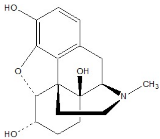
6alpha-Oxymorphone
